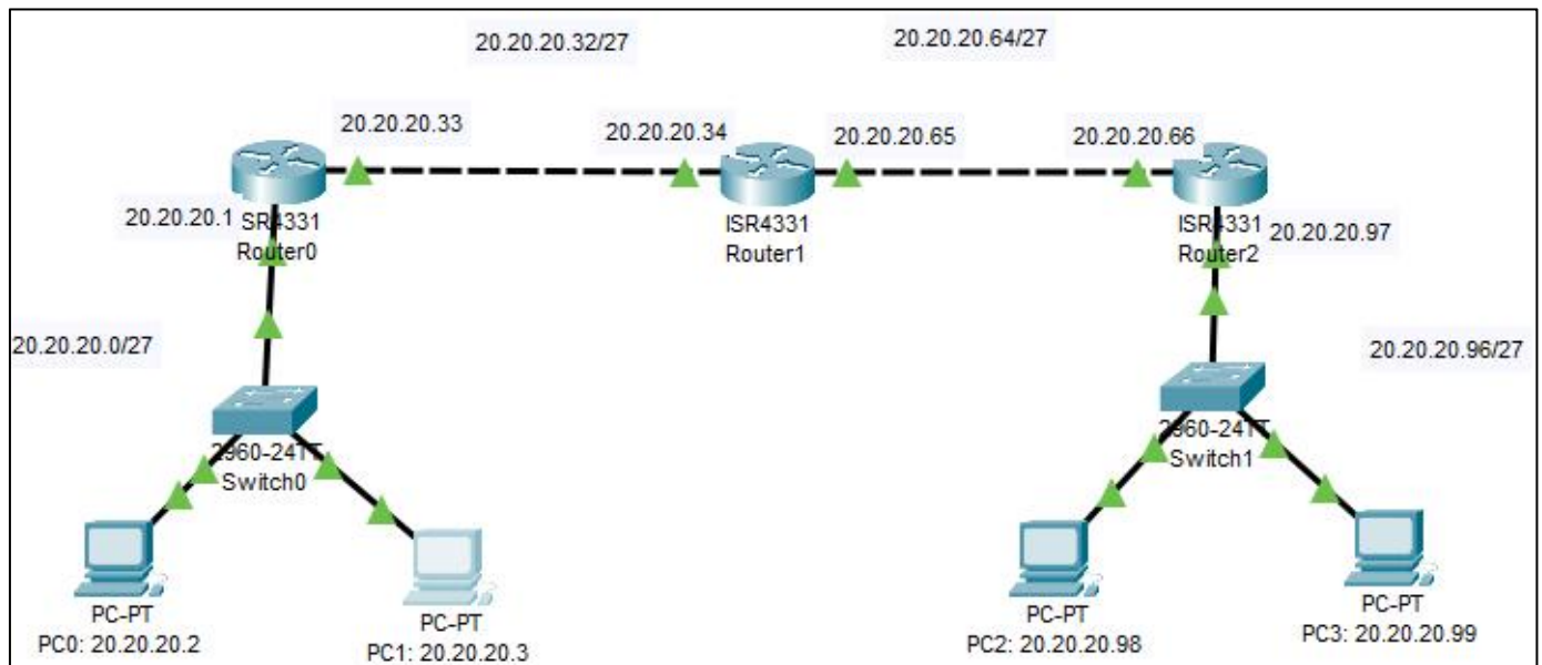
Fig: Topology of the Network
